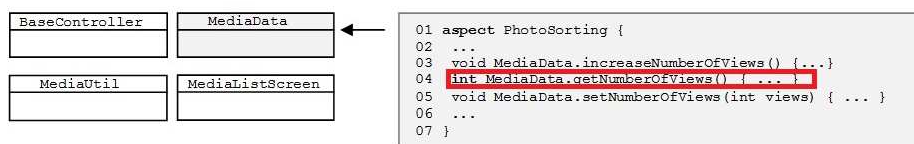
Figure 3.5: AspectJ example
