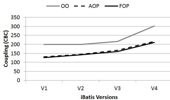
Figure 3.1: Modularity for iBatis
