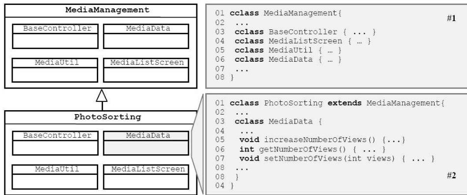
Figure 3.4: CaesarJ example of MobileMedia
