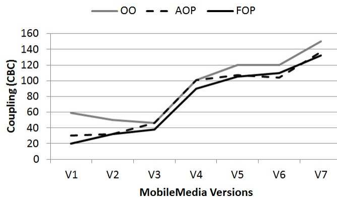
Figure 3.2: Modularity for MobileMedia
