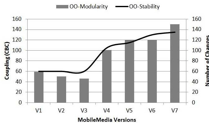
Figure 3.10: Modularity vs Stability for OO
