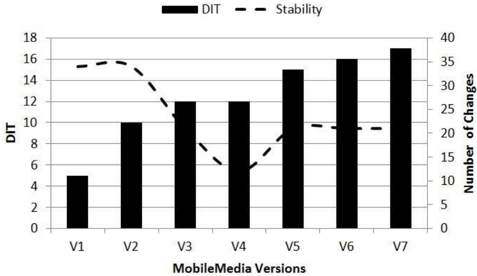
Figure 3.11: DIT vs Stability for CaesarJ
