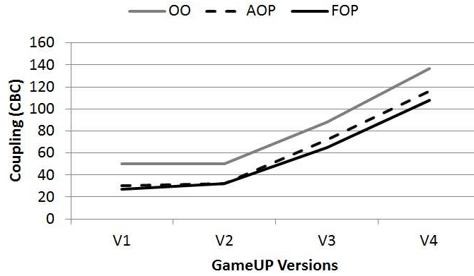
Figure 3.3: Modularity for Games
