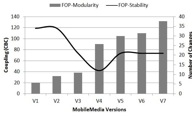
Figure 3.9: Modularity vs Stability for Caesar.J
