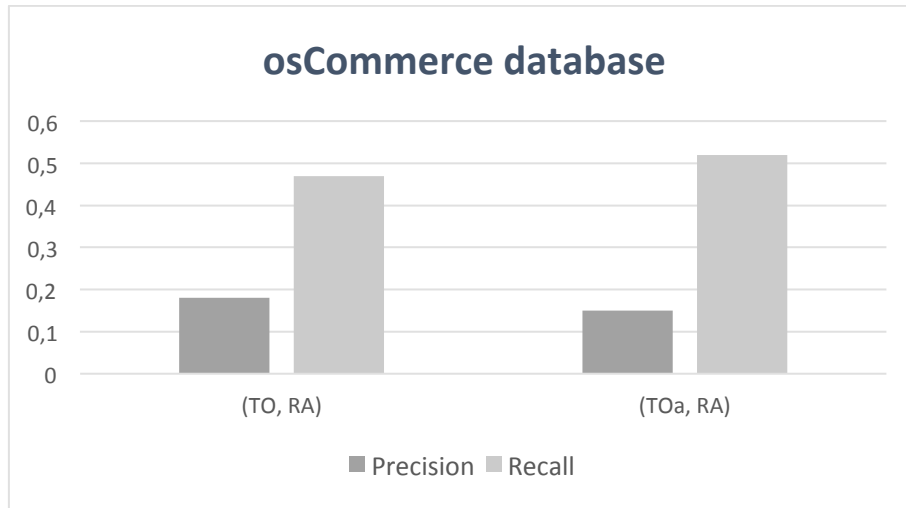
Figure 4.5 – osCommerce database results
