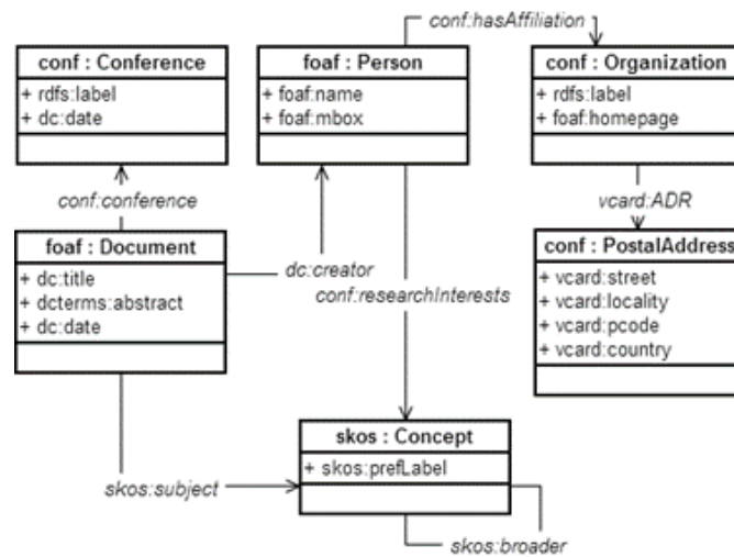
Figure 5.3 - ISWC_RDF exported ontology schema.
