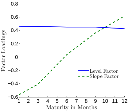
Figure 2.5: Factor loadings for South Africa
