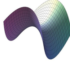
Figure 3.2: Hyperbolic paraboloid.
