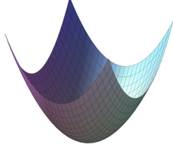
Figure 3.1: Elliptic paraboloid.
