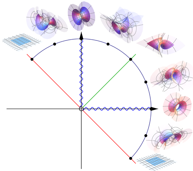
Figure 4.4: Deformation of minimal surfaces with planar curvature lines [8].
