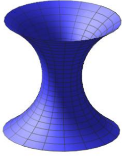
Figure 2.2: Catenoid.
