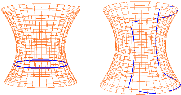
4.28(a): Curva - 1 4.28(b): Curva - 2
