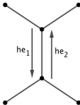
Figura 2.1: Half-Edge
