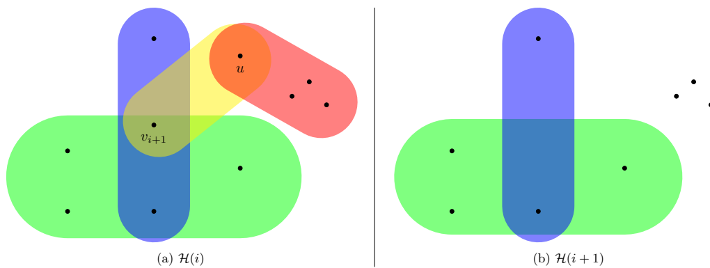
Figure 4.4: When the vertex v_{i+1} is chosen, notice that the vertex u is deleted and then the red edge that contained u is also deleted.
