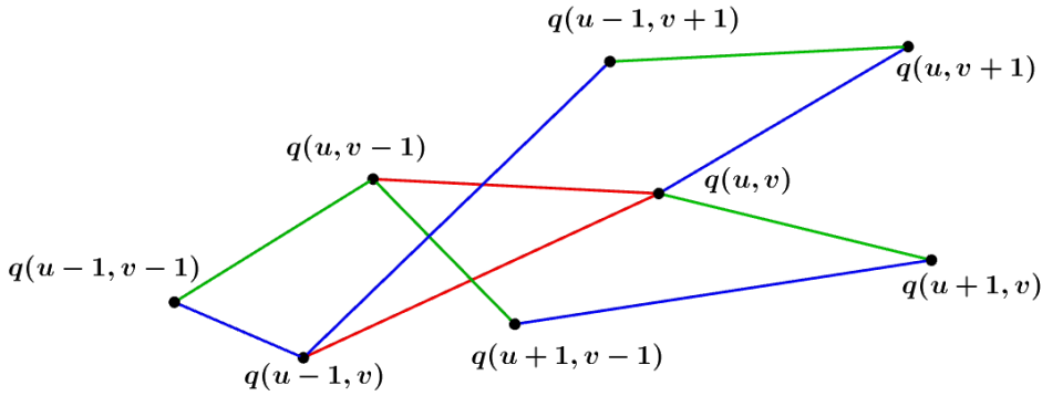
Figure 4.12: Swallowtail point.
