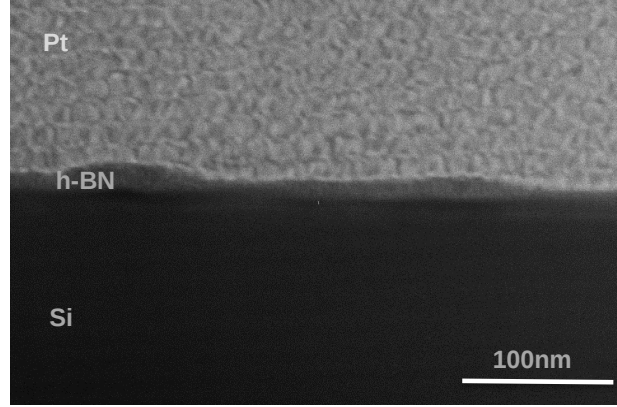
Figure 7.10: Cross-section STEM image of h-BN film depicting an h-BN film, overlaid with a 100 nm thick platinum (Pt) coating, grown on a Si \langle 100 \rangle substrate, following a 10-minute growth period at 1373 K.
