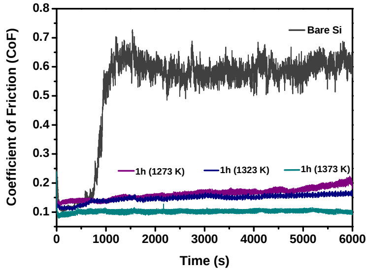
Figure 6.14: Presents the results obtained from the tribology test conducted on the Si <100> substrate and Si coated with h-BN (h-BN/Si) samples grown at 1 hour at 1273, 1323, and 1373 K, respectively. Under linear reciprocating ball-on-disc test. The test involved a constant sliding speed of 10 mm/s, a 10 mm sliding distance, and a corresponding Hertzian pressure of 398 MPa, displaying the variation of the coefficient of friction (CoF) with time (s).
