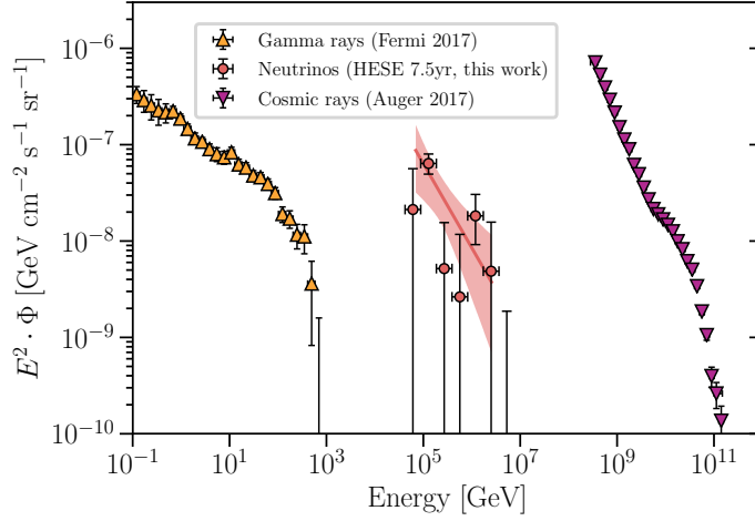
Figure 1.16: High-energy fluxes of gamma rays, neutrinos, and CRs. The high-energy gamma ray measurements by Fermi (17) are shown in orange, while the ultra-high energy cosmic ray measurements by the PAO (18) are shown as purple data points. Figure from (19)
