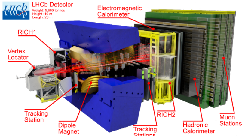
Figure 4.2: The LHCb detector 3D layout, including all its subdetectors.
