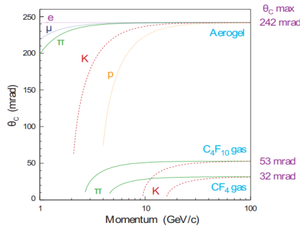
Figure 3.9: Cherenkov angle versus particle momentum for the RICH detectors [36].
