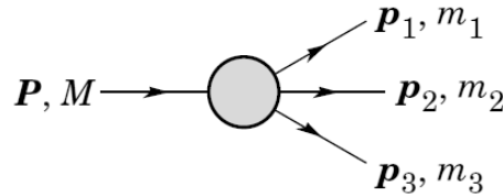
Figure 2.6: Schematic of a three-body decay [14].
