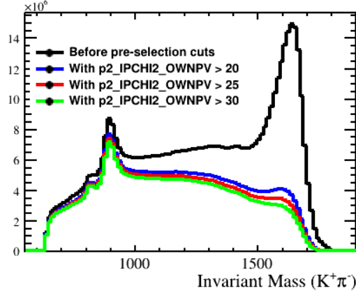
Figure 4.8: Two-body invariant mass reconstructed for the pair m_{3,1} with different values of \chi^2_{IP,2} requirements applied.
