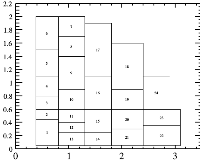
Figure A.1: Physics motivated binning scheme for the D^+ \rightarrow \pi^- \pi^+ K^+ Dalitz Plot.
