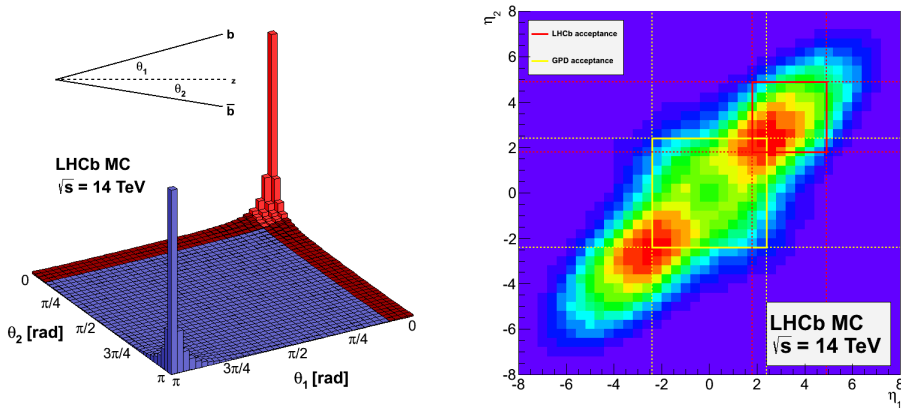
Figure 3.3: Distribution of b\bar{b} production as a function of the angle with respect to the beam axis (left) and as a function of the pseudorapidity (right) at \sqrt{s} = 14 TeV, created using PYTHIA8 and CTEQ6 NLO considering all the five flavours ( u, d, s, c, b ) in the PDFs and including the processess, weighted according to their cross-sections, q\bar{q} \rightarrow b\bar{b} , g\bar{g} \rightarrow b\bar{b} , q\bar{q} \rightarrow b\bar{b}g (where q \neq b ), b\bar{b} \rightarrow b\bar{b}g and g\bar{g} \rightarrow b\bar{b}g [38].
