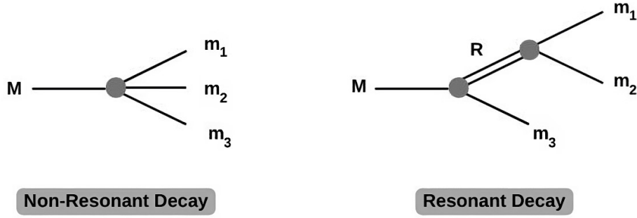
Figure 2.8: Representation of a non-resonant and a resonant tree-body decay.
