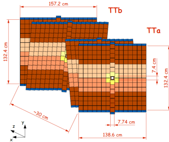
Figure 3.7: Schematic view of the four layers of the Trigger Tracker stations [41].
