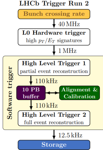
Figure 3.14: Overview of the LHCb trigger system [46].
