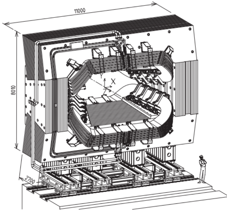
Figure 3.6: Illustration of LHCb magnet dipole [36]
