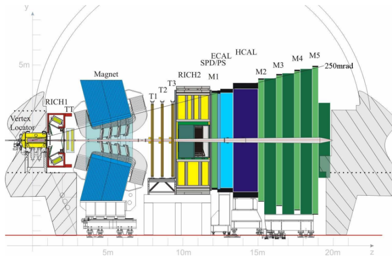
Figure 3.4: Illustration of LHCb detector components [36].
