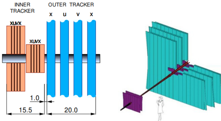
Figure 3.8: Schematic representation of the top view of a tracking station (left) with dimensions along the beam axis given in cm [42] and illustration of the trajectory stations (right) with the IT (purple) and the OT (blue) [41].
