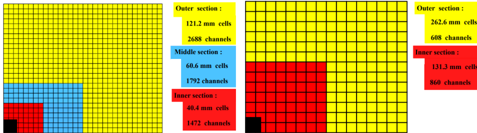
Figure 3.12: Illustration of the SPD/PS and ECAL detectors (left) and HCAL (right). One quarter of the detector front face is shown [44].
