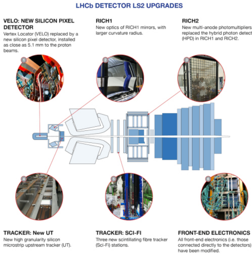
Figure 3.16: LHCb Upgrade I summary [48].
