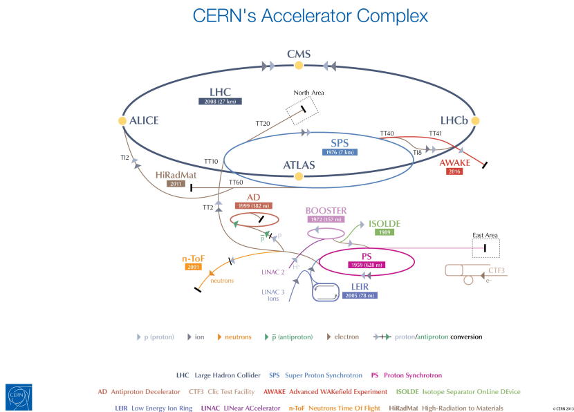
Figure 3.1: CERN accelerator complex [32]
