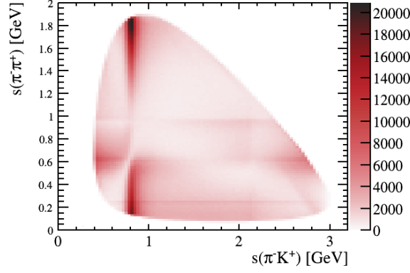
Figure 4.19: Dalitz plot of the final sample full mass spectrum (left) and 2\sigma_{eff} signal region (right) of D^+ \rightarrow \pi^-\pi^+K^+ .
