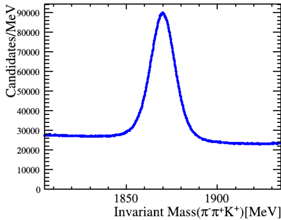
Figure 4.16: D^+ \rightarrow \pi^- \pi^+ K^+ mass distribution after all the selection requirements.
