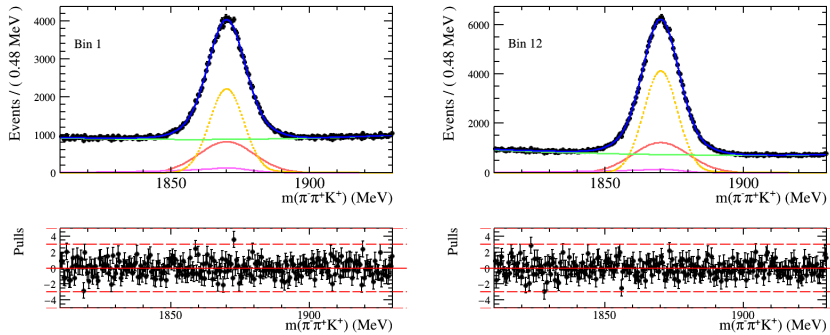
Figure 5.2: Invariant mass fit of bin 1 of sample 1 (left) and bin 12 of sample 2 (right), used on the fit-per-bin method.
