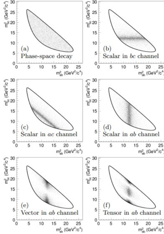
Figure 2.9: Example Dalitz plots for a decay M \rightarrow m_a m_b m_c with (a) phase-space decay, (b-d) one scalar resonance appearing in various decay channels, (e, f) vector and tensor resonances. Adapted from [30].
