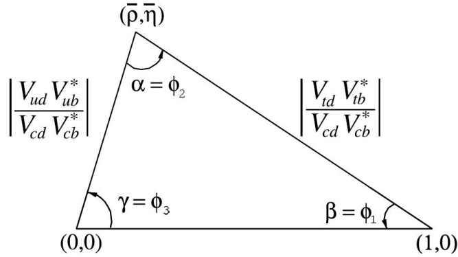
Figure 2.2: Sketch of the unitary triangle [22].
