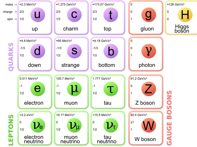
Figure 2.1: Standard Model of Elementary Particles representation [10].
