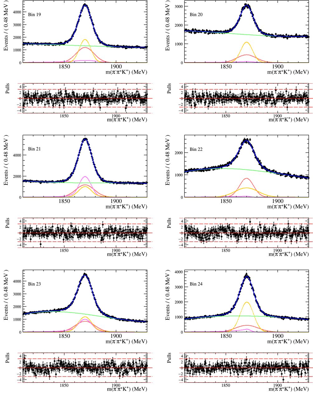
Figure A.5: D^+ \rightarrow \pi^- \pi^+ K^+ invariant mass fit per bin of the physics motivated binning scheme with 24 total bins in sample 1 (bins 19-24).
