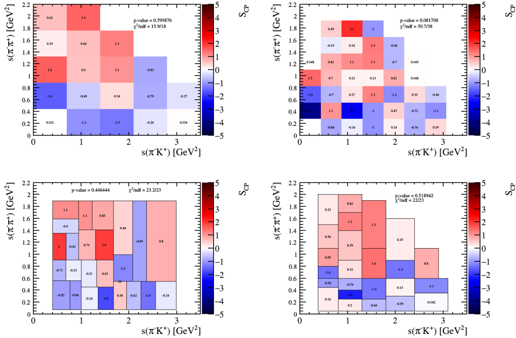
Figure 5.6: D^+ \rightarrow \pi^- \pi^+ K^+ background test using standard event counting in each bin for uniform 5 \times 5 grid (top left), uniform 8 \times 8 grid (top right), adaptive with 25 bins (bottom left) and physics motivated with 24 bins (bottom right).
