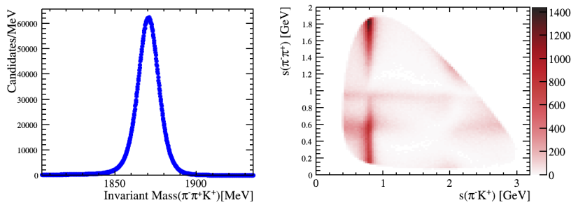
Figure 4.9: Mass distribution and Dalitz plot for the MC sample after the selection criteria.
