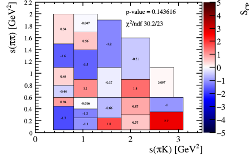
Figure 5.4: D^+ \rightarrow \pi^- \pi^+ K^+ null test using the fit-per-bin method for the physics motivated binning with 24 bins.
