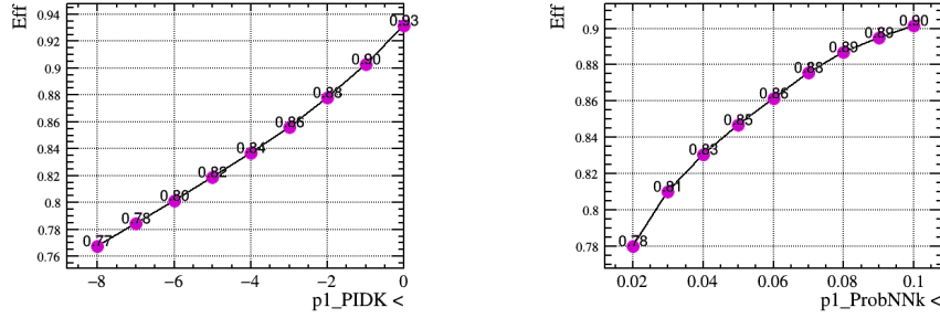
Figure 4.5: Signal efficiency associated to each value of p1\_PIDK and p1\_ProbNNk requirements.
