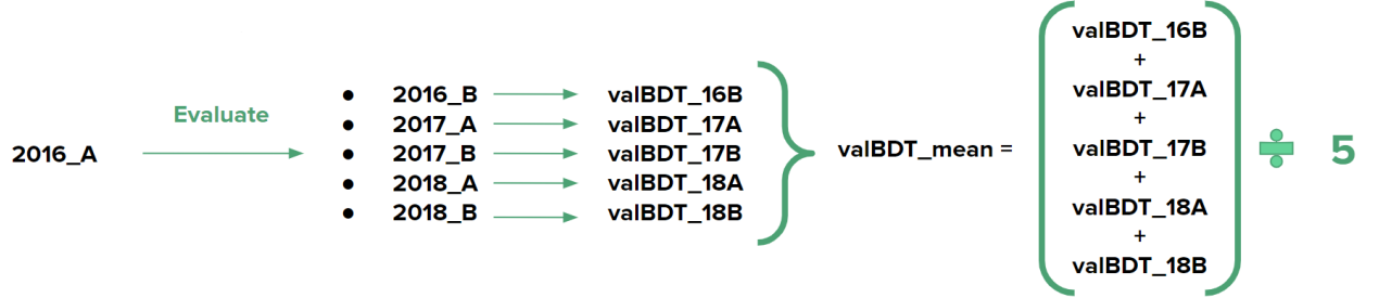
Figure 4.14: Schematic representation of the construction of the BDT classifier.
