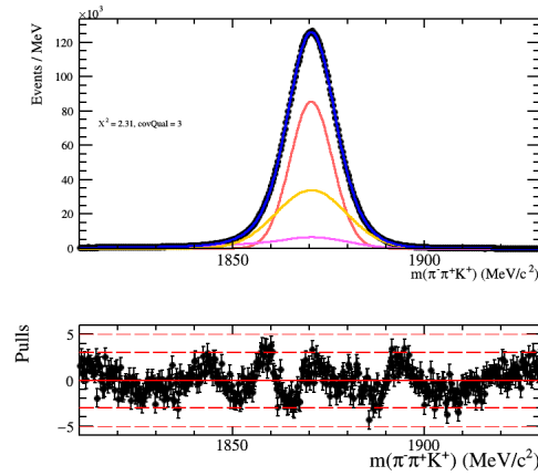
Figure 4.17: Monte Carlo fit using the PDF in Eq. 4-2.
