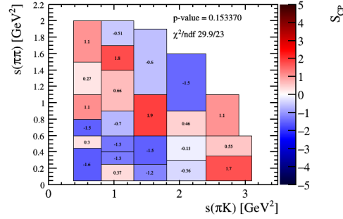
Figure 5.5: D^+ \rightarrow \pi^- \pi^+ K^+ background test using the fit-per-bin method for the physics motivated binning with 24 bins.
