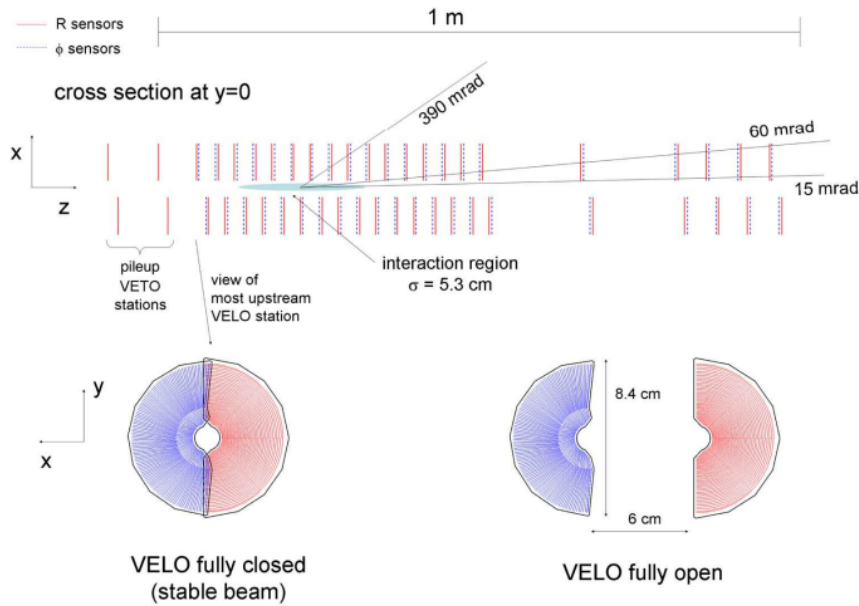
Figure 3.5: Schematic representation of the VELO detector and cross section. The z direction is defined along the beam axis into the detector, y is vertical and x is horizontal [36].
