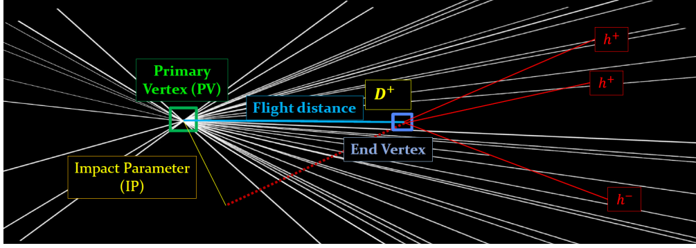
Figure 4.1: Illustration of a D^+ \rightarrow h^- h^+ h^+ decay at LHCb. Courtesy of my dear friend Felipe Almeida.
