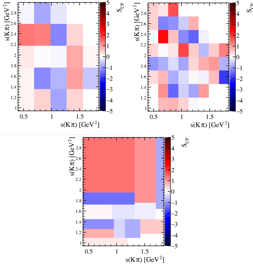
Figure 5.9: \mathcal{S}_{CP} distribution for the control channel D^+ \rightarrow K^- \pi^+ \pi^+ using 5 \times 5 grid (top left) and 8 \times 8 grid (top right) for the uniform and 25 bins (bottom) for the adaptive binning scheme.
