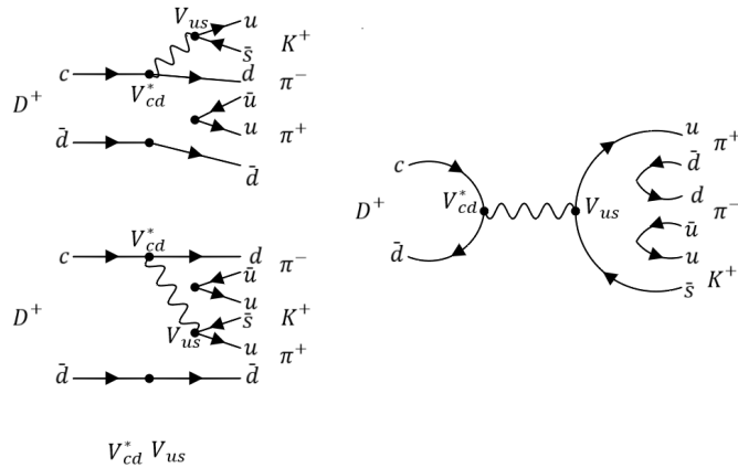
Figure 2.4: D^+ \rightarrow \pi^- \pi^+ K^+ topologies: tree-level emission of W (top left), tree-level emission of W colour suppressed (bottom left) and annihilation diagram (Right).
