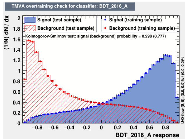
Figure 4.13: BDT response for training and testing samples of 2016_A.
