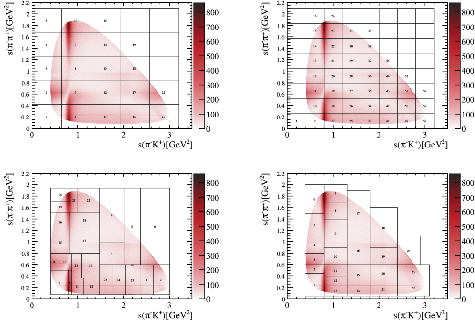
Figure 5.1: DP binning schemes plotted for the events of the D^+ \rightarrow \pi^- \pi^+ K^+ final sample signal region. Uniform 5 \times 5 grid (top left), uniform 8 \times 8 grid (top right), adaptive with 25 bins (bottom left) and physics motivated with 24 bins (bottom right). The binning configuration number is shown.
