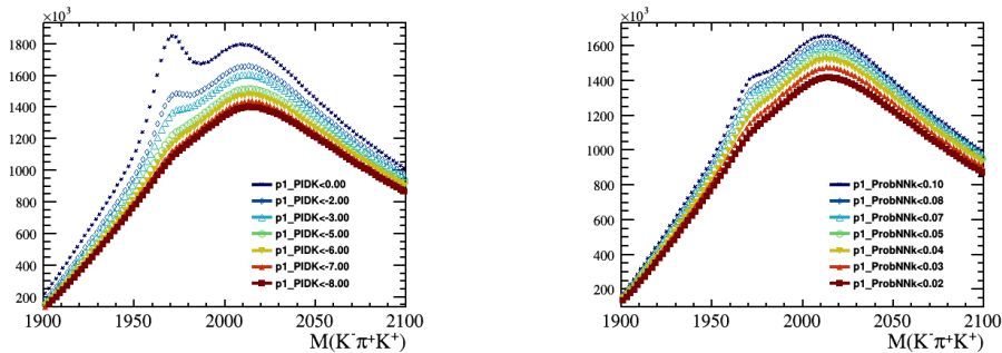
Figure 4.3: Three-body invariant mass reconstructed by assigning a kaon mass to particle 1 ( \pi^- ), for multiple values of p1\_PIDK and p1\_ProbNNk requirements.
