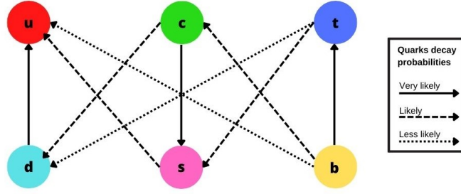
Figure 2.3: Probabilities of quarks decay proportional to |V_{ij}|^2 .
