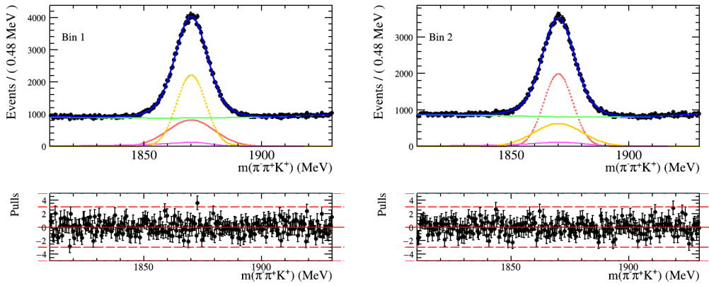
Figure A.2: D^+ \rightarrow \pi^- \pi^+ K^+ invariant mass fit per bin of the physics motivated binning scheme with 24 total bins in sample 1 (bins 1 and 2).
