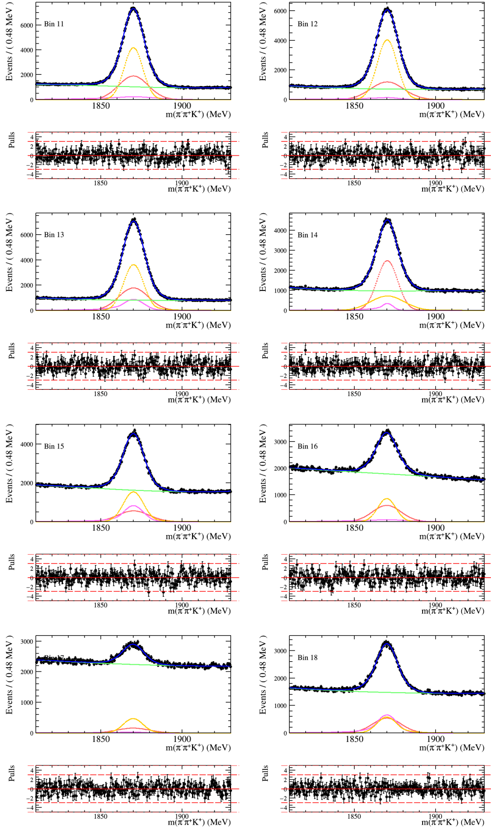
Figure A.4: D^+ \rightarrow \pi^- \pi^+ K^+ invariant mass fit per bin of the physics motivated binning scheme with 24 total bins in sample 1 (bins 11-18).
