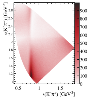
Figure 5.8: Dalitz plot for one sample of the control channel D^+ \rightarrow K^- \pi^+ \pi^+ .
