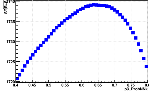
Figure 4.6: Significance calculated for different requirements of p3_ProbNNk.
