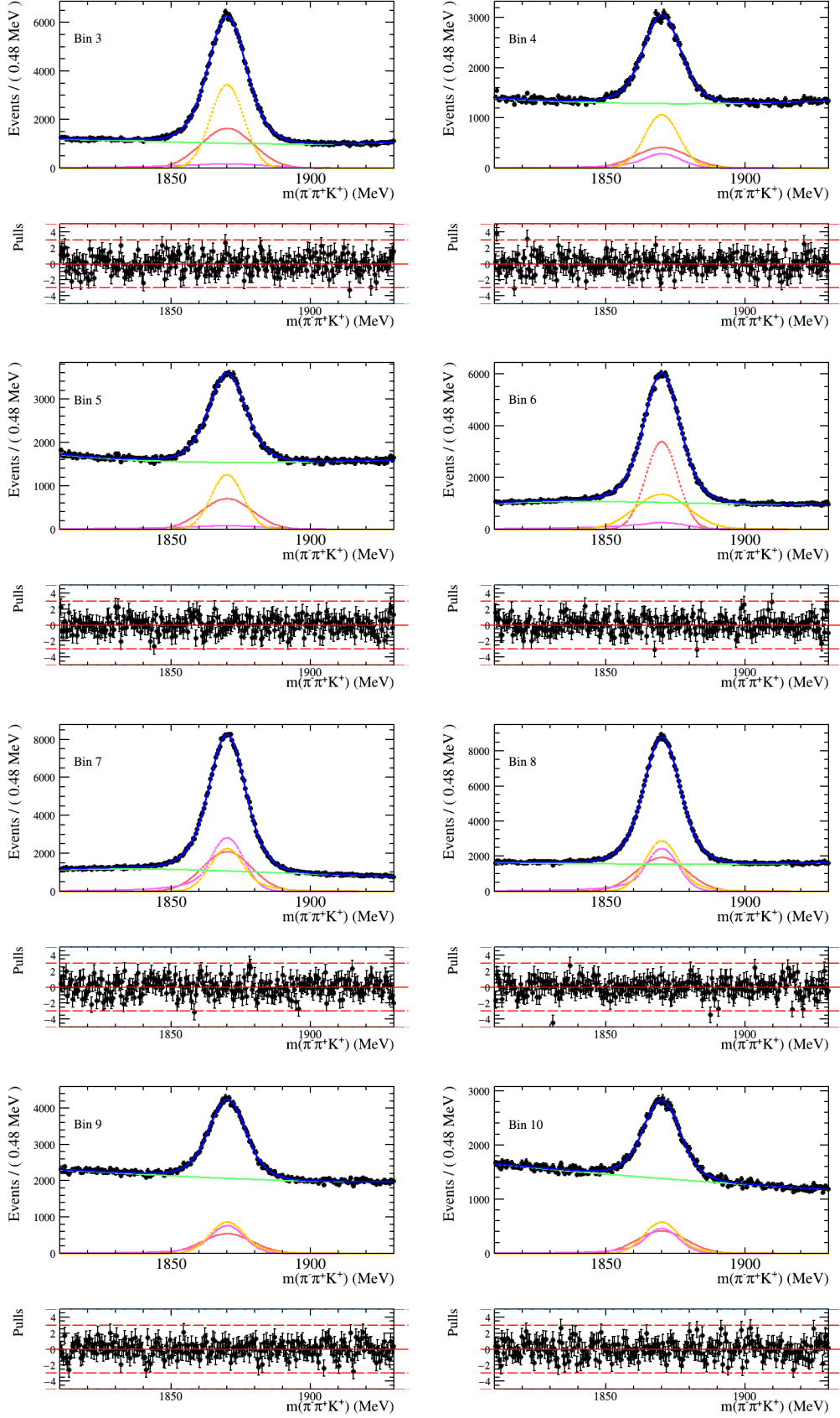
Figure A.3: D^+ \rightarrow \pi^- \pi^+ K^+ invariant mass fit per bin of the physics motivated binning scheme with 24 total bins in sample 1 (bins 3-10).
