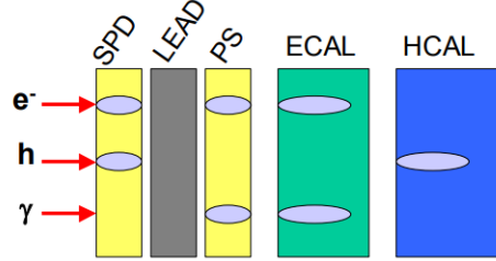
Figure 3.11: Signal deposited on all the parts of the calorimeter by an electron, a hadron, and a photon [45].
