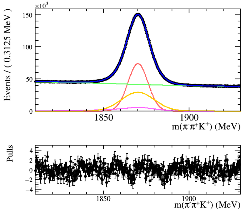
Figure 4.18: Mass fit of D^+ \rightarrow \pi^- \pi^+ K^+ final sample..
