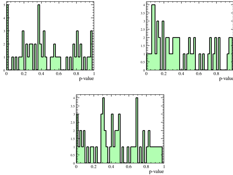
Figure 5.10: Distribution of p -value responses over the search in all samples of the control channel for uniform 5 \times 5 grid (top left) and 8 \times 8 grid (top right) and adaptive with 25 bins (bottom).
