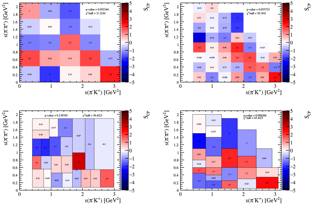
Figure 5.3: D^+ \rightarrow \pi^- \pi^+ K^+ null test counting all entries in the bin (standard Mirandizing test), for uniform 5 \times 5 grid (top left), uniform 8 \times 8 grid (top right), adaptive with 25 bins (bottom left) and physics motivated with 24 bins (bottom right).
