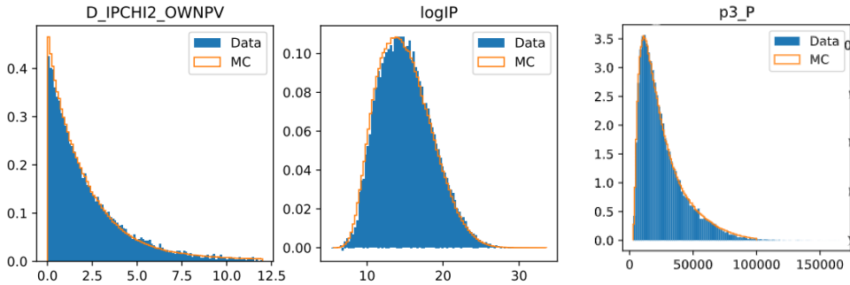
Figure 4.11: \chi^2_{IP,D} , log IP and p3\_P distributions for D^+ \rightarrow \pi^- \pi^+ K^+ signal decays after the reweight process.
