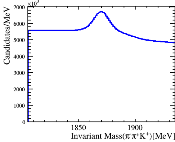
Figure 4.2: D^+ \rightarrow \pi^- \pi^+ K^+ mass distribution.
