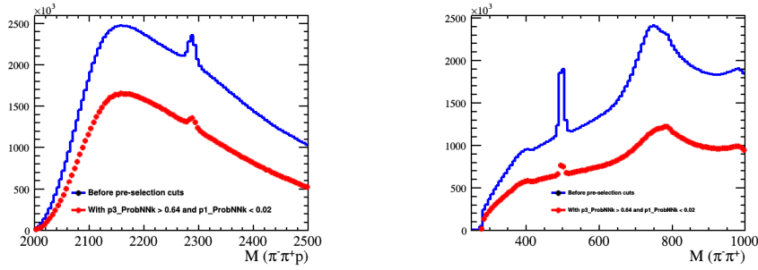
Figure 4.7: Invariant mass reconstruction assigning a proton mass to particle 3 ( K^+ ) for the \Lambda_c^+ \rightarrow \pi^- \pi^+ p contamination (left) and the invariant mass for the pair \pi^- \pi^+ for the D^+ \rightarrow K_s^0 K^+ contamination (right).
