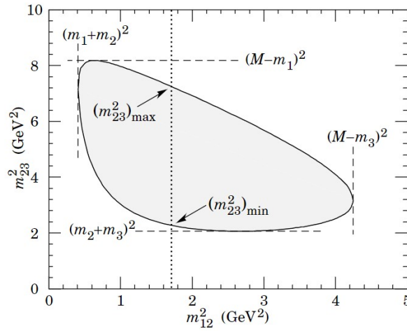
Figure 2.7: Generic Dalitz plot for a three-body final state [14].
