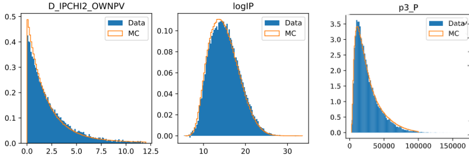
Figure 4.10: \chi^2_{IP,D} , log IP and p3\_P distributions for D^+ \rightarrow \pi^- \pi^+ K^+ signal decays before the reweight process.
