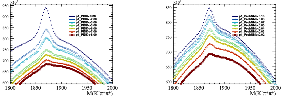
Figure 4.4: Three-body invariant mass reconstructed by assigning a kaon mass to the particle 1 ( \pi^- ) and a pion mass to particle 3 ( K^+ ), for multiple values of p1\_PIDK and p1\_ProbNNk requirements.
