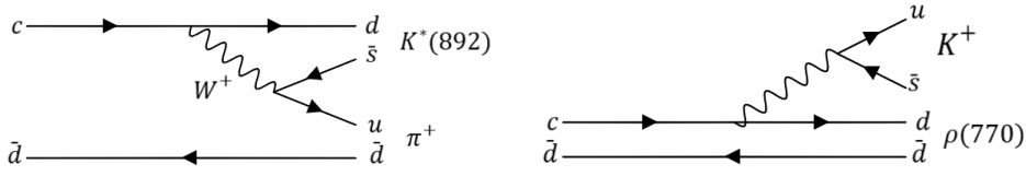
Figure 2.5: D^+ \rightarrow \pi^-\pi^+K^+ with main resonances highlighted.
