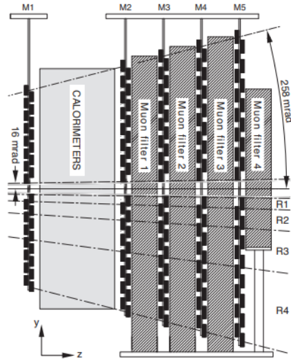
Figure 3.13: Schematic representation of the muon system side-view [36].
