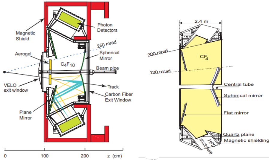
Figure 3.10: Side view of the schematic layout of RICH1 (left) and top view of the schematic of RICH2 [36].
