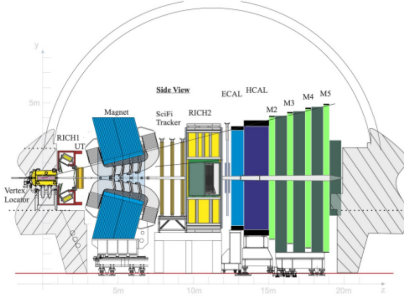
Figure 3.15: Side view of the layout of the upgraded LHCb detector [47].
