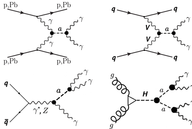
Figure 2.6: Representative diagrams of ALPs searches at the LHC via exclusive diphotons (toptleft), diphotons from vector-boson-fusion (with V = \gamma, Z , top right), exotic triphoton Z-boson decays (bottom left), and exotic 4-photon Higgs-boson decays (bottom right) [3].
