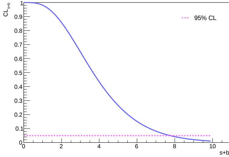
Figure 4.2: The CL_{s+b} curve for 1000 values of s + b between 0 and 10. At s + b = 7.75 , the probability of observing n_{obs} = 3 events or less is 5%. At this point, we can get the s_{up} from the subtraction of the given background.
